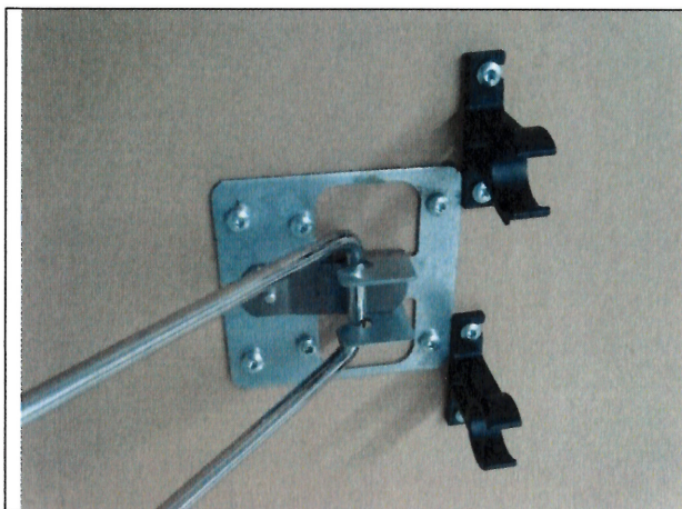
Pic.3: Lock mechanism
