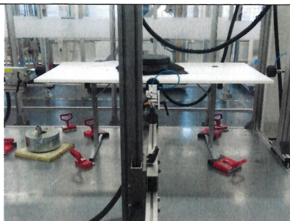
Pic.8: Horizontal static load test
